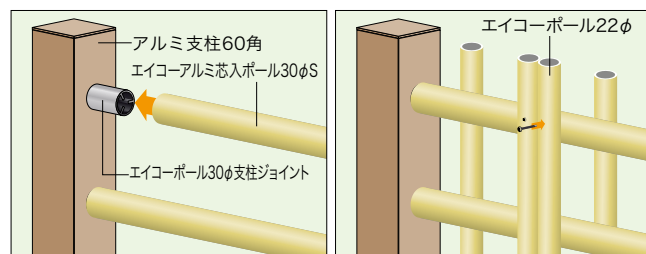
[四ツ目垣取付図]
