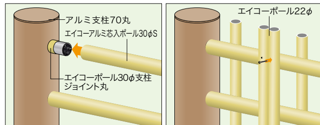
[四ツ目垣取付図]
